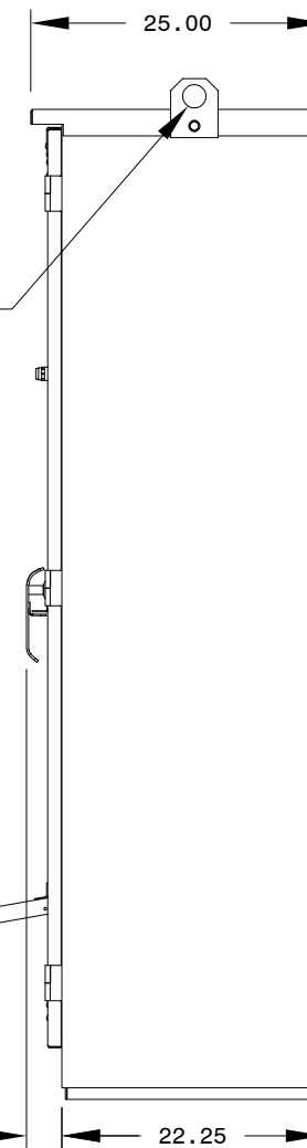
SIDE ELEVATION
