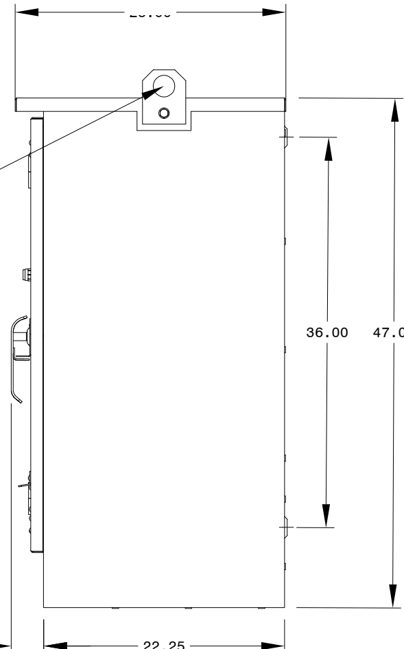
SIDE ELEVATION
