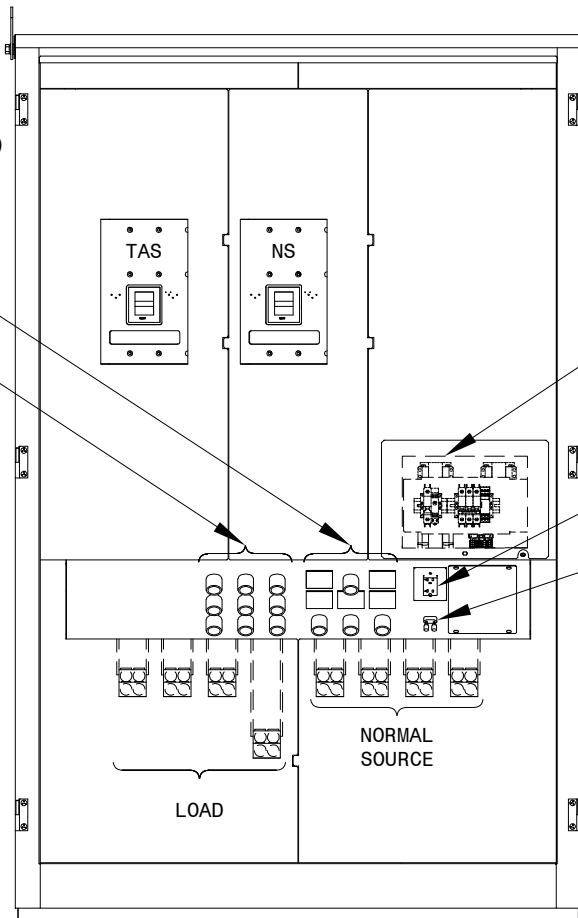
FRONT ELEVATION DOORS REMOVED
