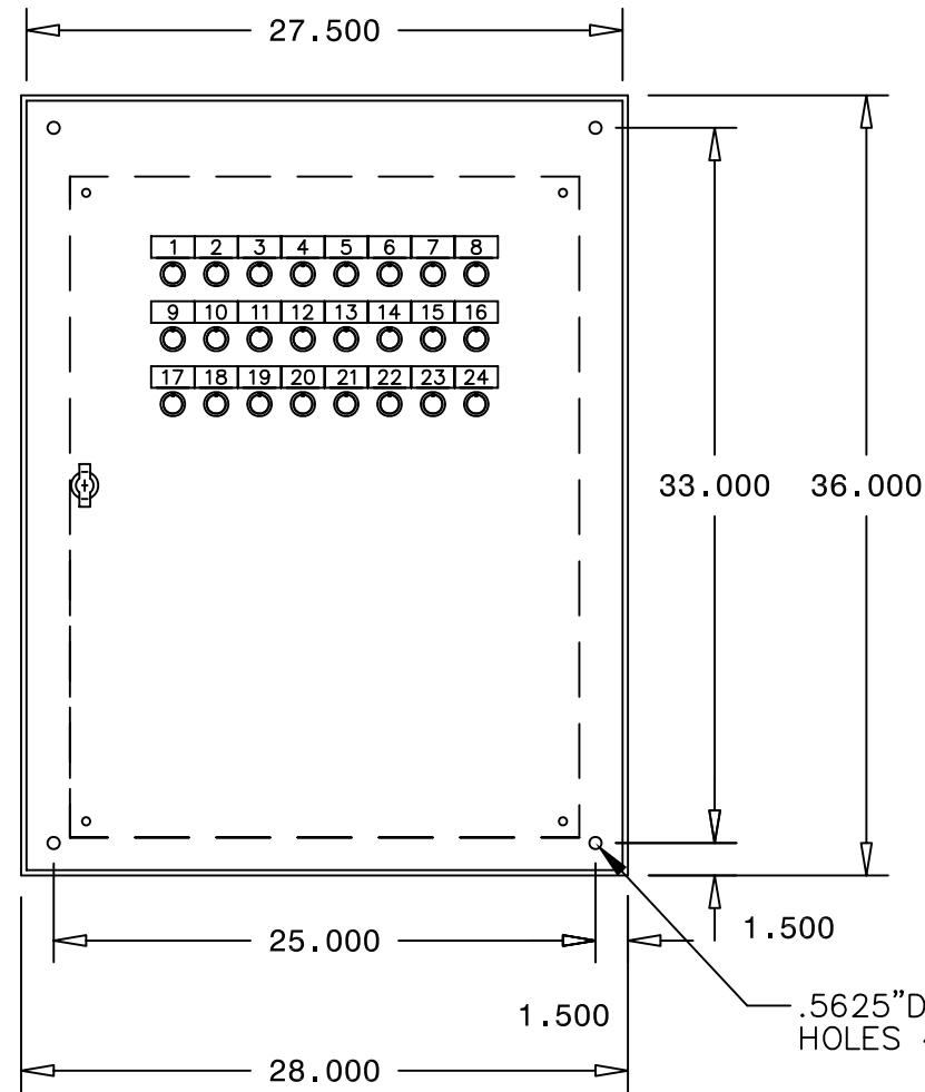
FRONT VIEW
