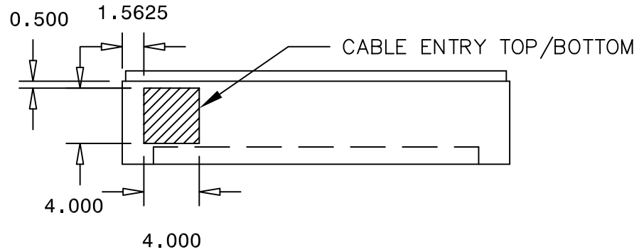
BOTTOM VIEW (Recommended Cable Access Areas)
